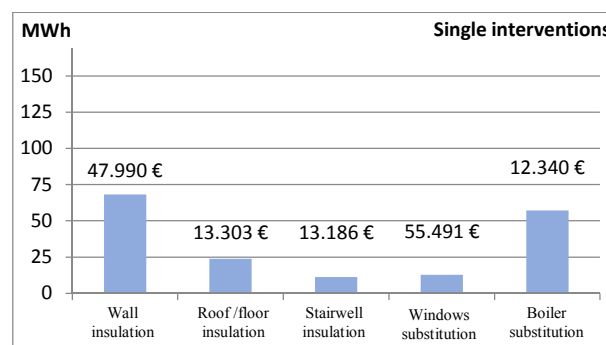
Fig. 2. Energy savings and costs of single interventions: corso Vercelli.
